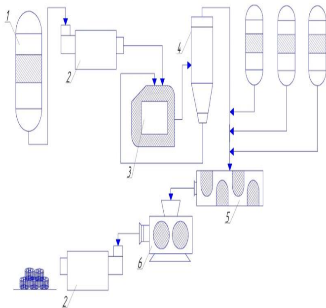
Figure 1 Technological scheme of production of coal briquettes
