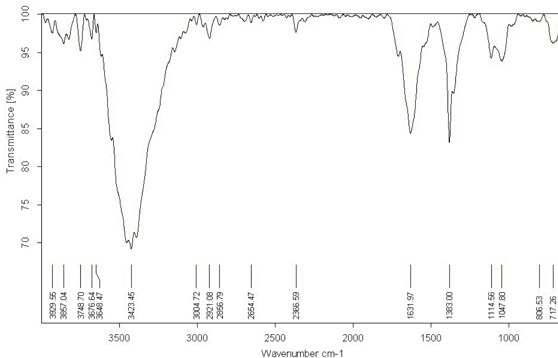
Figure (4): FT-IR spectrum of GONPs at (300\text{ °C}) by chemical method.
