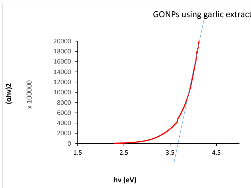
Figure (3): Energy band gap of GONPs using garlic extract.
