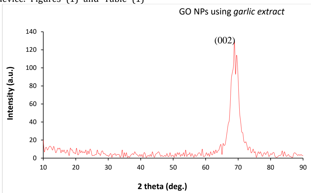
Figure 1. X-ray diffraction (XRD) patterns of graphene oxide nanoparticles (GONPs) prepared using garlic extract.
