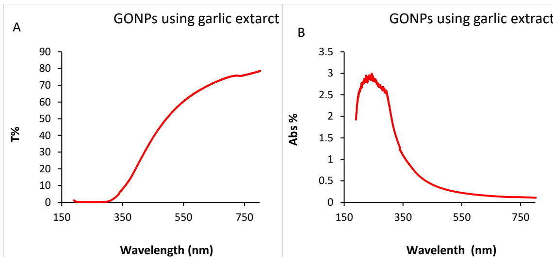
Figure (3): UV-visible spectrum of GONPs, (A-B) using garlic extract.
