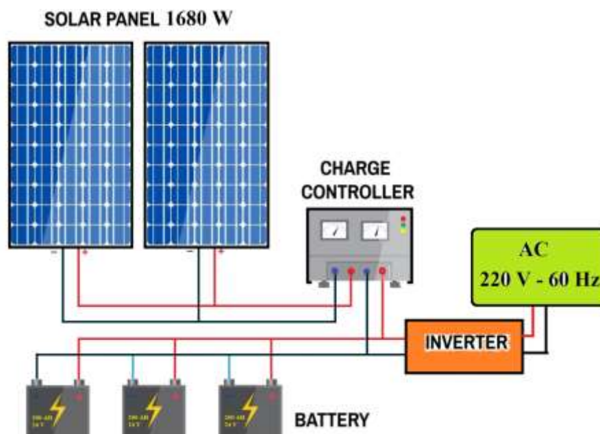
Figure ( 5 ) Connect the components of the photovoltaic system
