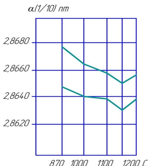
Previous quenching temperatures. °C Fig. 2. Change in the grating period of steel U8A depending on the temperature of Previous quenching and intermediate tempering
