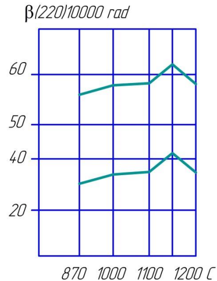
Previous quenching temperatures, °C Fig. 1. Change in the parameters of the structure of steel U8A depending on the previous quenching and medium tempering.
