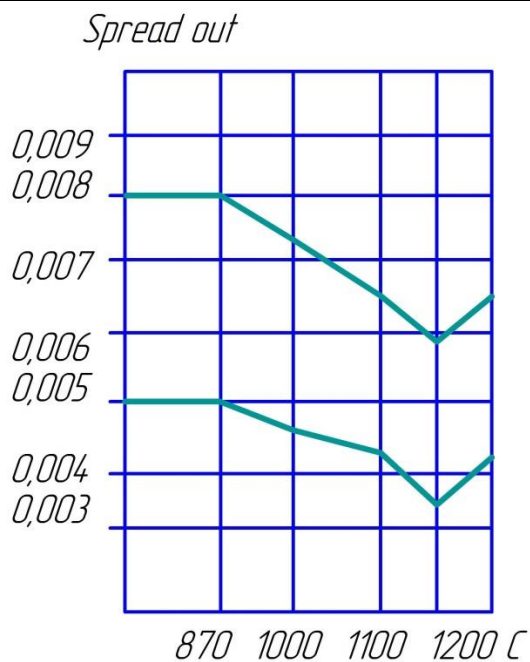
Previous quenching temperatures °C Figure 4. Change in wear out resistance depending on the Previous quenching temperature
